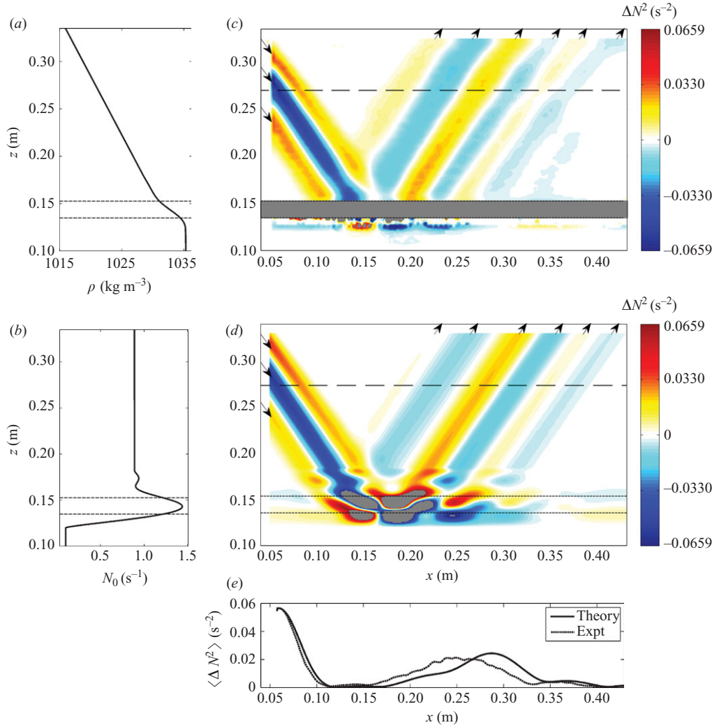
FIGURE 8. (a) Measured density profile. (b) Corresponding N_0 profile. (c) Experimental \Delta N^2 field obtained using synthetic Schlieren for \omega/N_1=0.82 . (d) Theoretical \Delta N^2 field obtained by numerically solving (3.3). Regions with values outside the limits of the colourbar or where experimental data were not reliable due to strong stratification are grey. The arrows indicate the direction of local energy propagation and the dashed lines indicate the horizontal section where the experimental and theoretical solutions are compared in (e). (e) Theoretical (solid) and experimental (dotted) amplitude envelopes of \Delta N^2 for the horizontal sections marked in (c) and (d).
